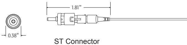
ST Connector
