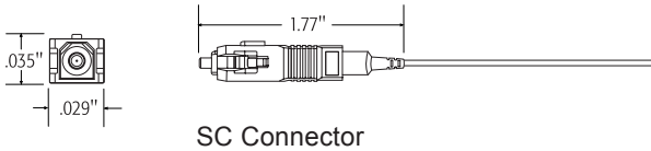
SC Connector
